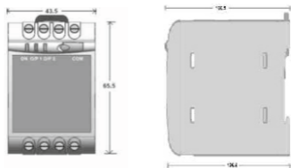
Fig. 6 Dimensional measurements
