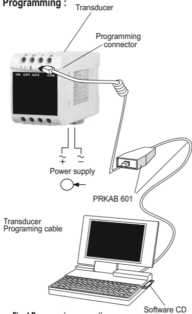
Fig. 4 Programming connection
